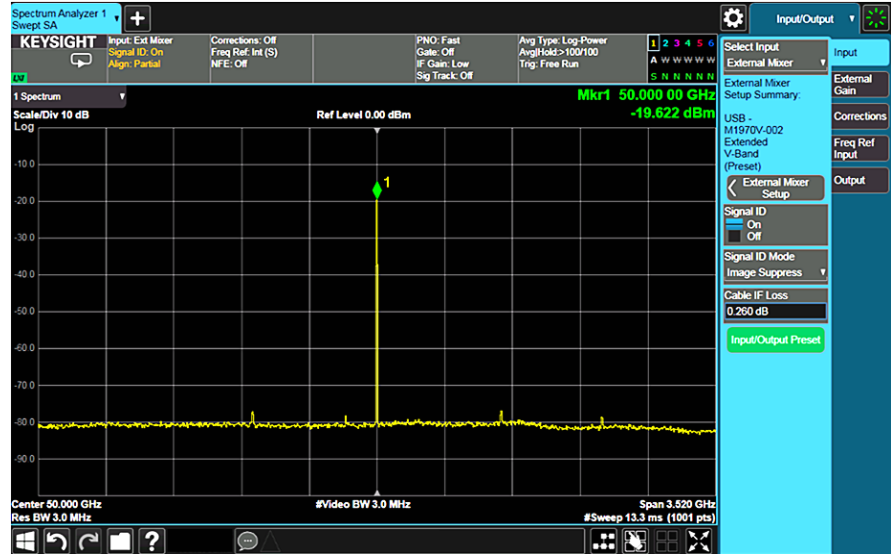
Figure 7-18. The image suppress function displays only real signals
