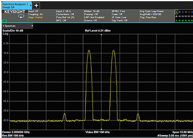
Figure 1-5. Two-tone test on an RF power amplifier
