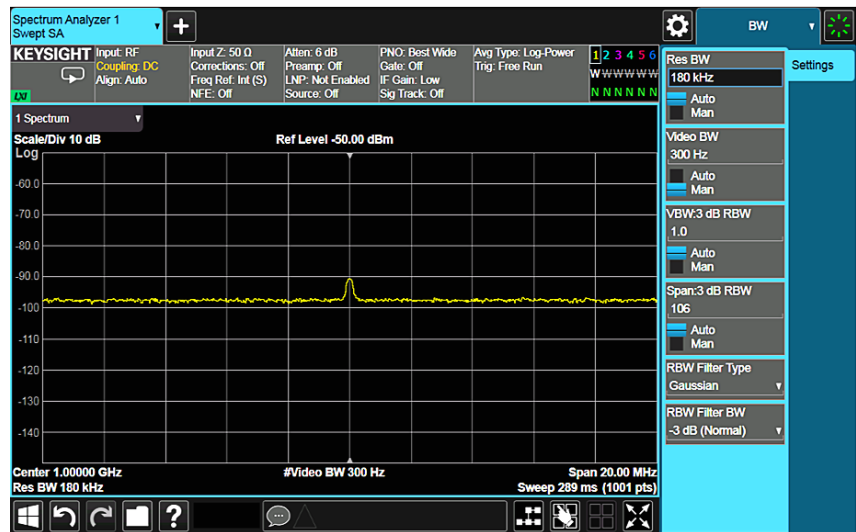
Figure 5-3. Video filtering makes low-level signals more discernible
