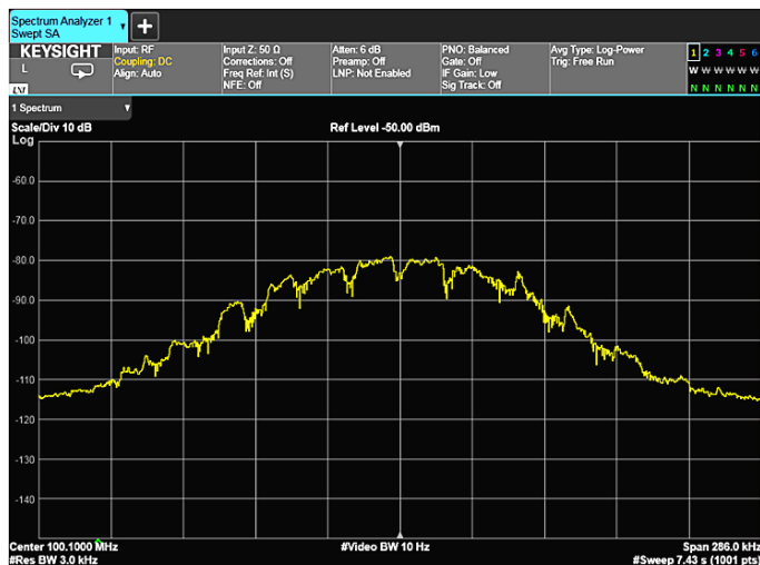
Figure 2-32a. Video filtering
