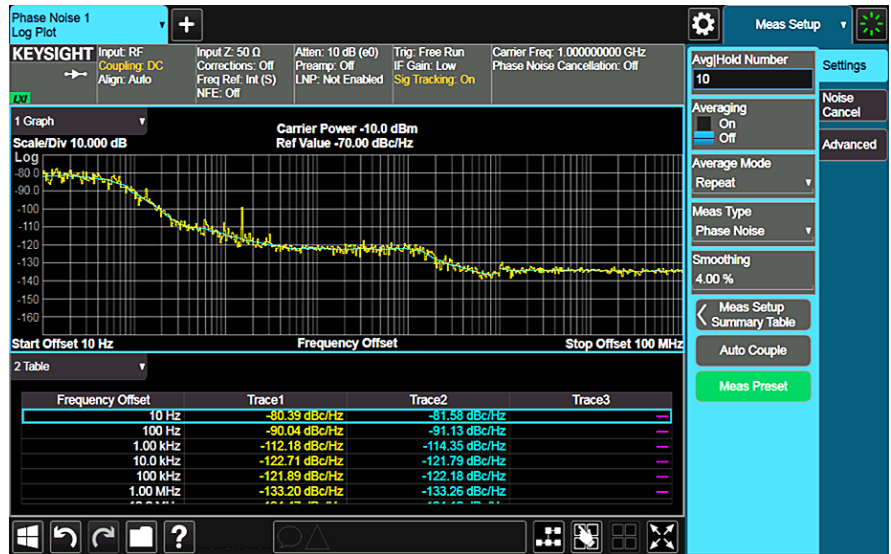
Figure 8-3. Phase noise measurement
