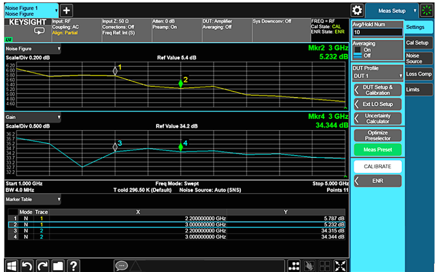
Figure 8-2. Noise figure measurement
