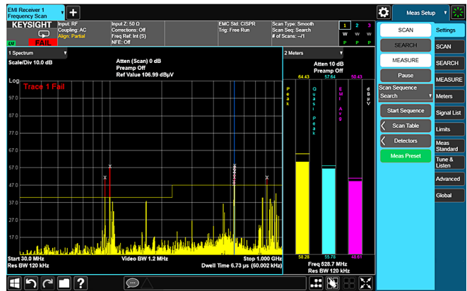
Figure 1-6. Radiated emissions plotted against CISPR11 limits as part of an EMI test
