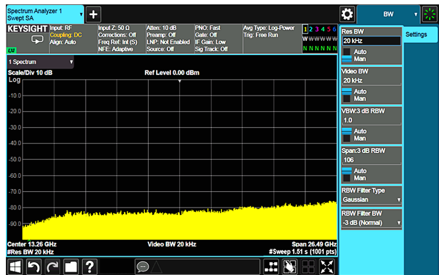
Figure 2-14b. Full span sweep speed, RBW of 20 kHz, with Option FS1
