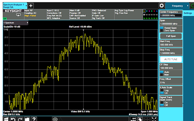
Figure 2-41. Spectrum of the GSM signal
