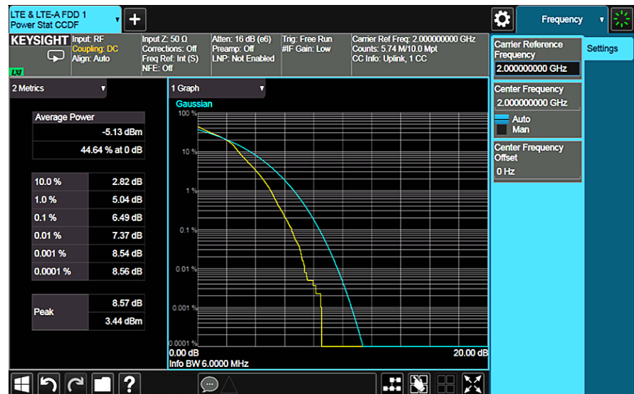
Figure 8-1. CCDF measurement
