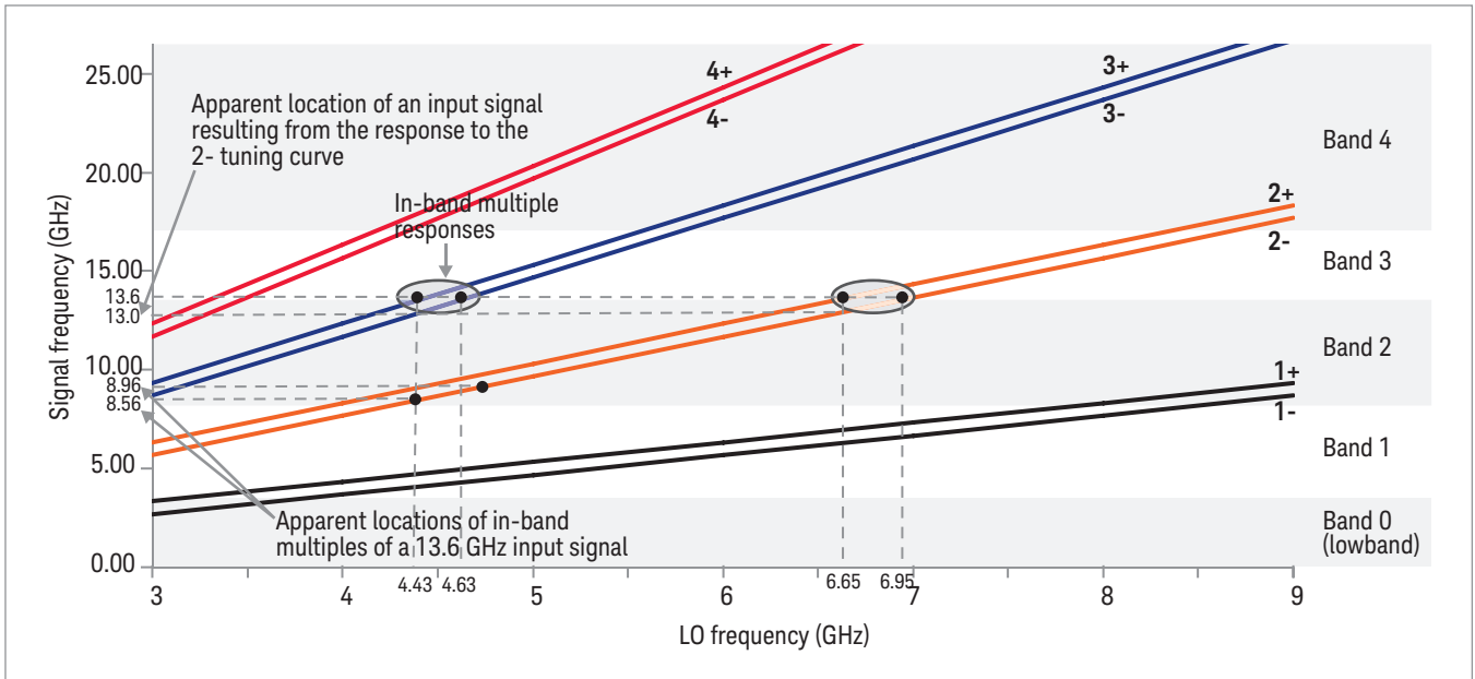
Figure 7-5. Tuning curves up to 4th harmonic of LO showing in-band multiple responses to a 13.6-GHz input signal
