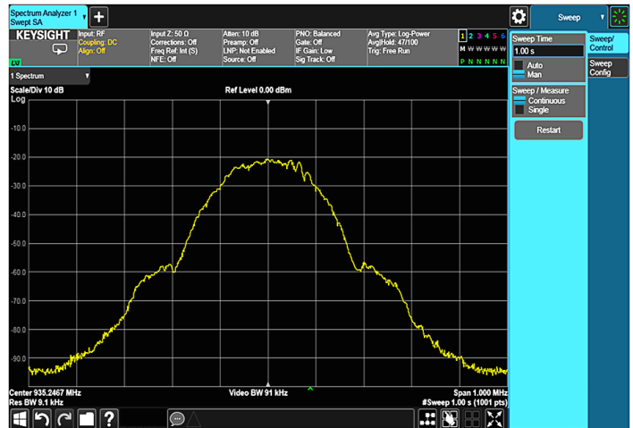
Figure 2-39. Spectrum of time slot 3 reveals that the spurious signal is not caused by this burst.
