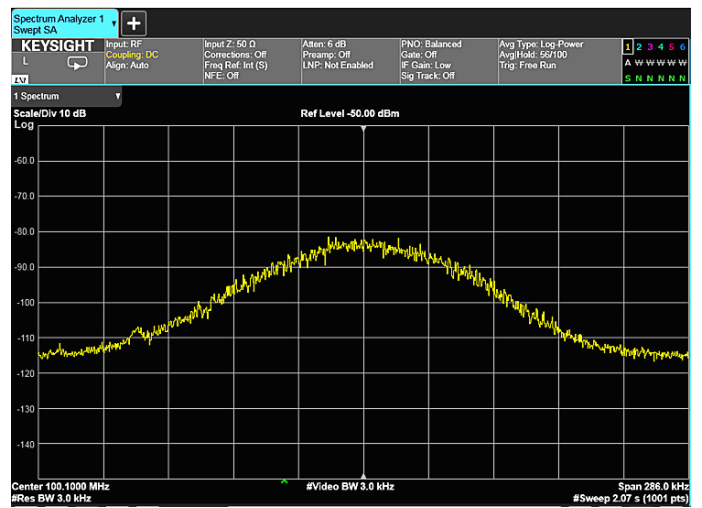
Figure 2-32b. Trace averaging
